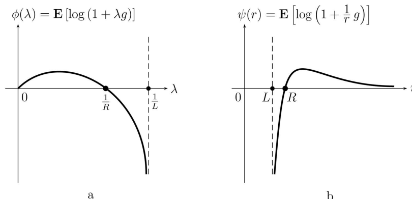
FIG. A1.—The functions \phi(\lambda) and \psi(r) (see lemma 1)
